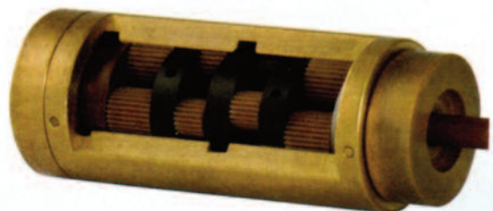
A custom design unit from Precipart incorporated a brass housing, Vespel gears and a beryllium copper retainer ring to test magnetic fields and study how they were disrupted by nonmagnetic entities (courtesy of Precipart).
